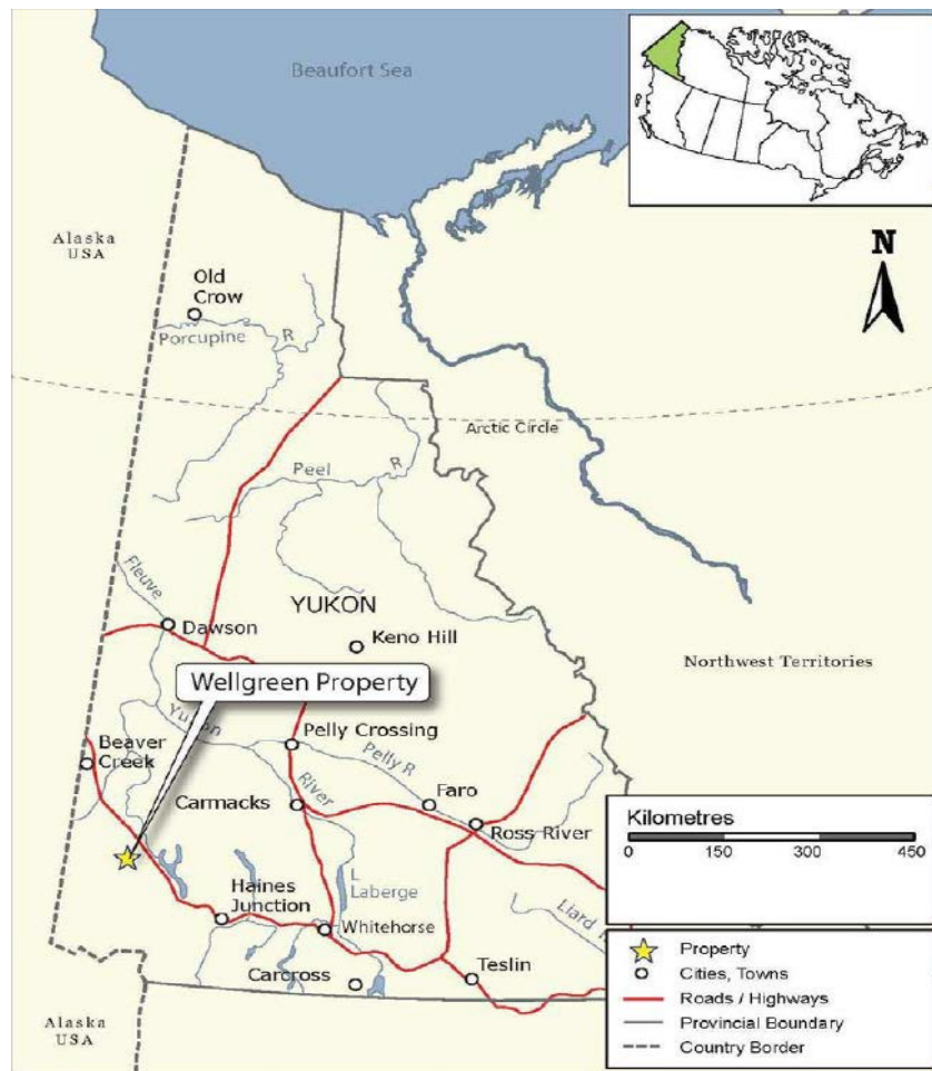
Figure 1-1: Wellgreen Platinum Location Map (GeoSim, Wellgreen 2015)
