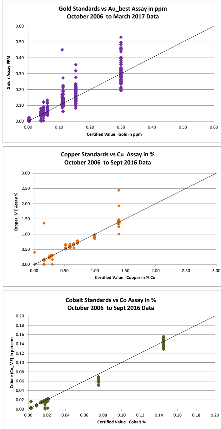
Figure 12-2: Standards Results, Au, Cu, Co
