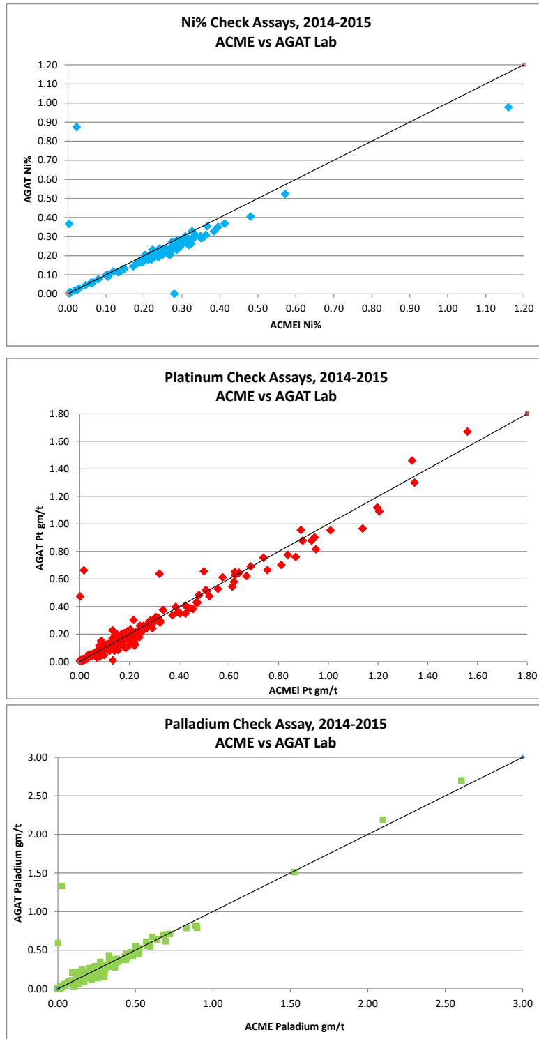
Figure 12-7: Check Assays, 2014-2015
