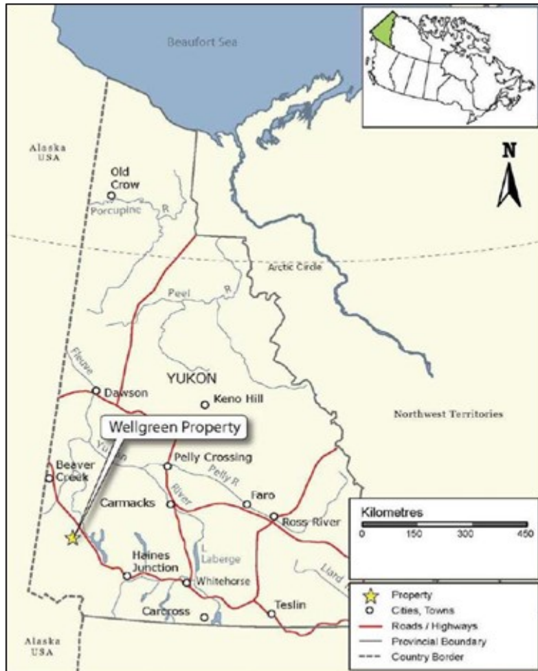
Figure 4-1: Wellgreen Platinum Location Map
