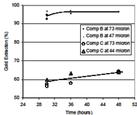
Figure 13.1 – Gold Leach Kinetics
