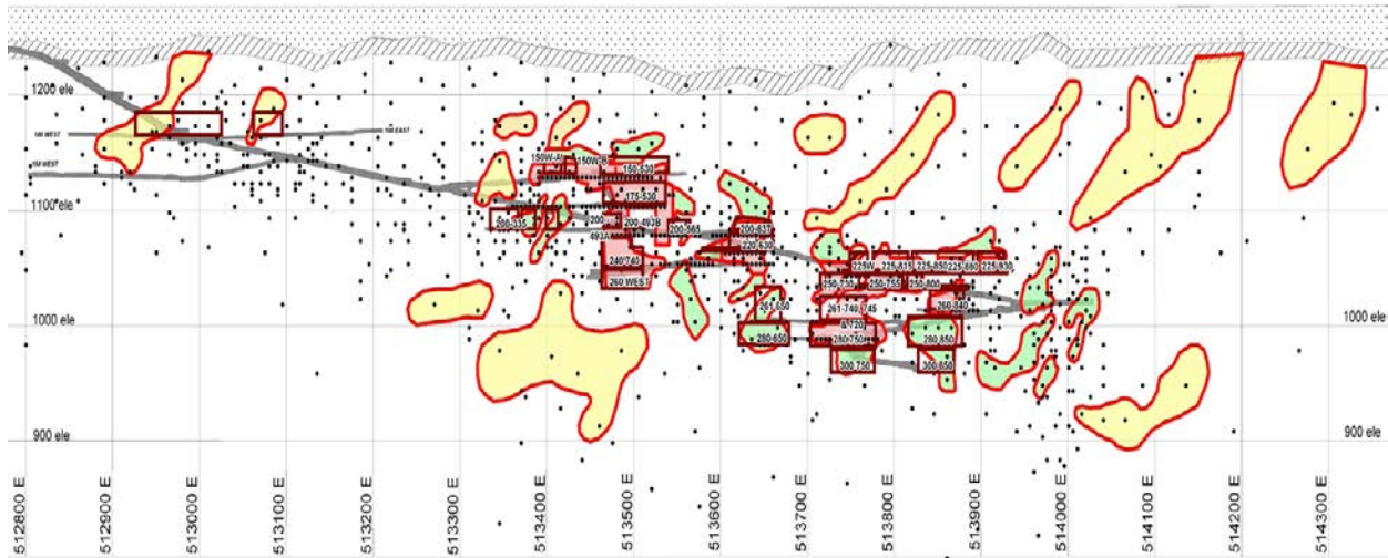
Figure 16.1 Clavos Longitudinal Section
