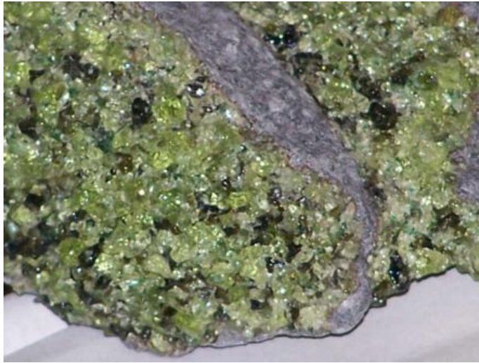
Photo D: Black Orthopyroxene (n.d.). Image referenced from https://en.wikipedia.org/wiki/Pyroxene
