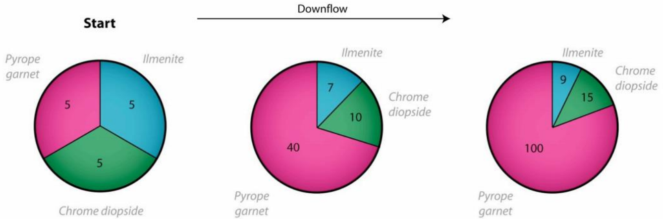
Diagram H: Downflow evolution of indicator mineral assemblages ... in which rapid break down of larger pyrope garnets produces abundant sand-sized grains. ... Numbers refer to grain counts. (Cummings et al. (2014))
