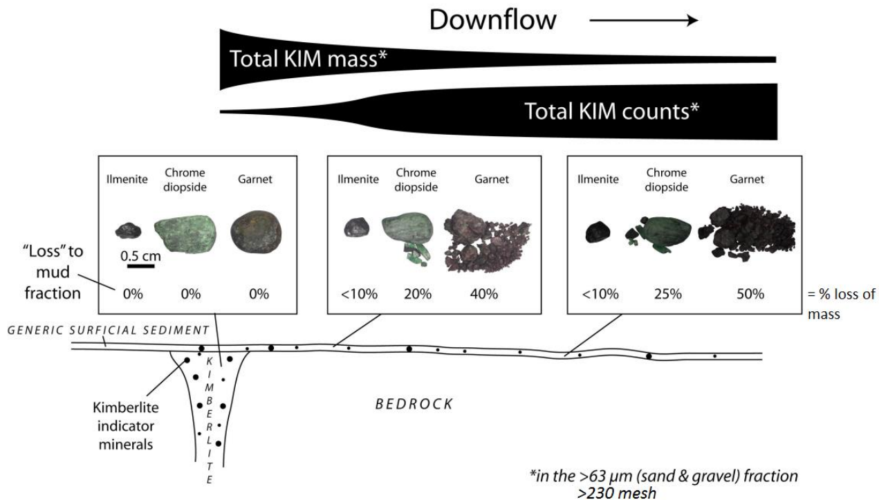
Diagram G: Farther downflow, total KIM counts would decrease, assuming continued comminution (in addition to selective sorting and/or dilution). (Cummings et al. (2014))
