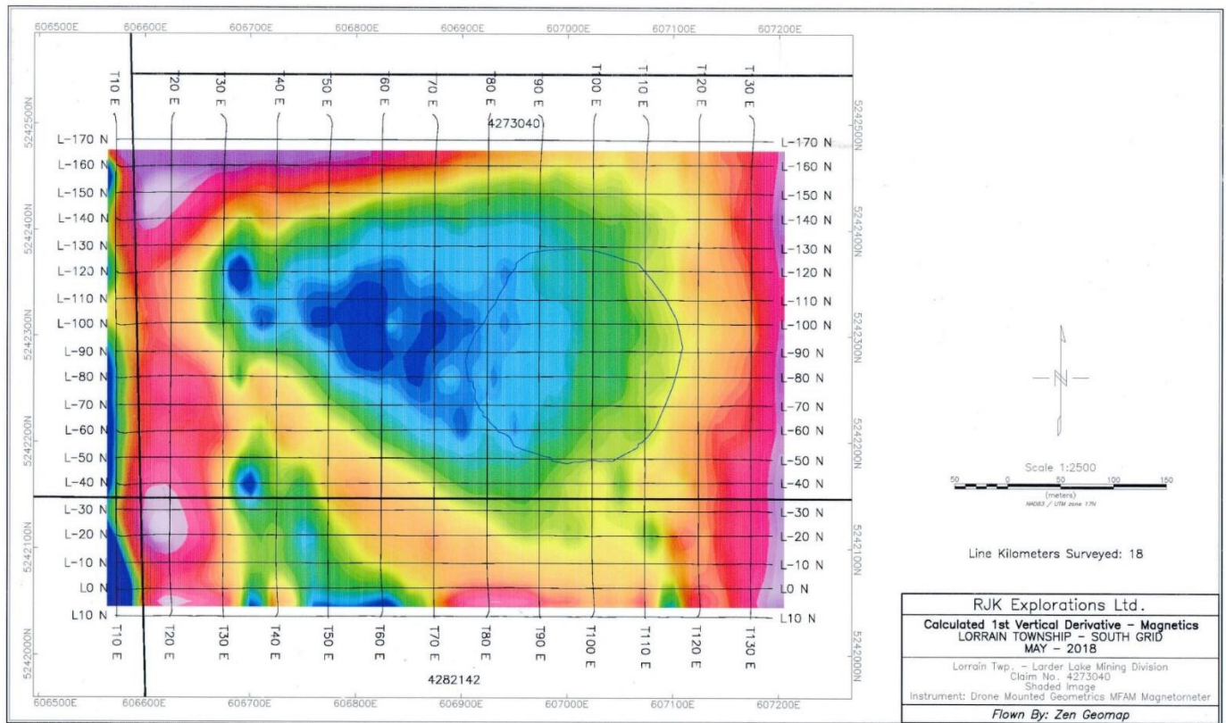
Figure 4: Calculated 1 st Vertical Derivative over Paradis Pond
