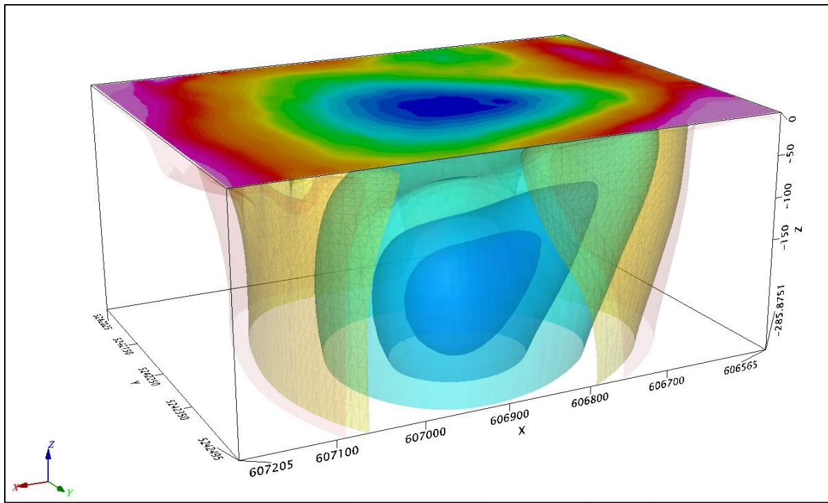
Figure 8: 3D Inversion showing negative isosurfaces in blue (looking azimuth 207 degrees/inclination 19 degrees), Paradis Pond
