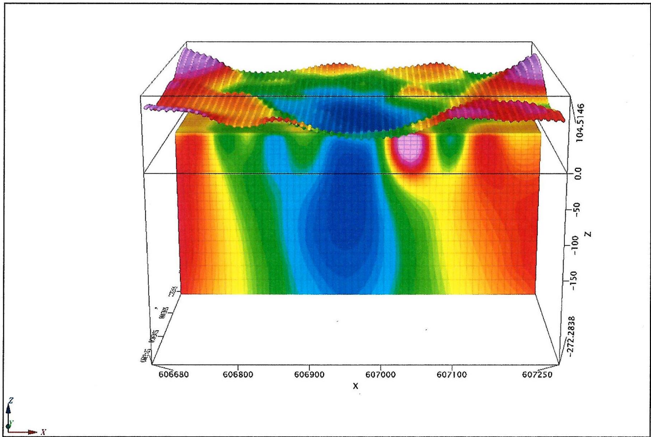
Figure 13: 3D Inversion Voxel with magnetic overlay looking North with section cut through 5243150N at 16-degree inclination, Cedar Pond
