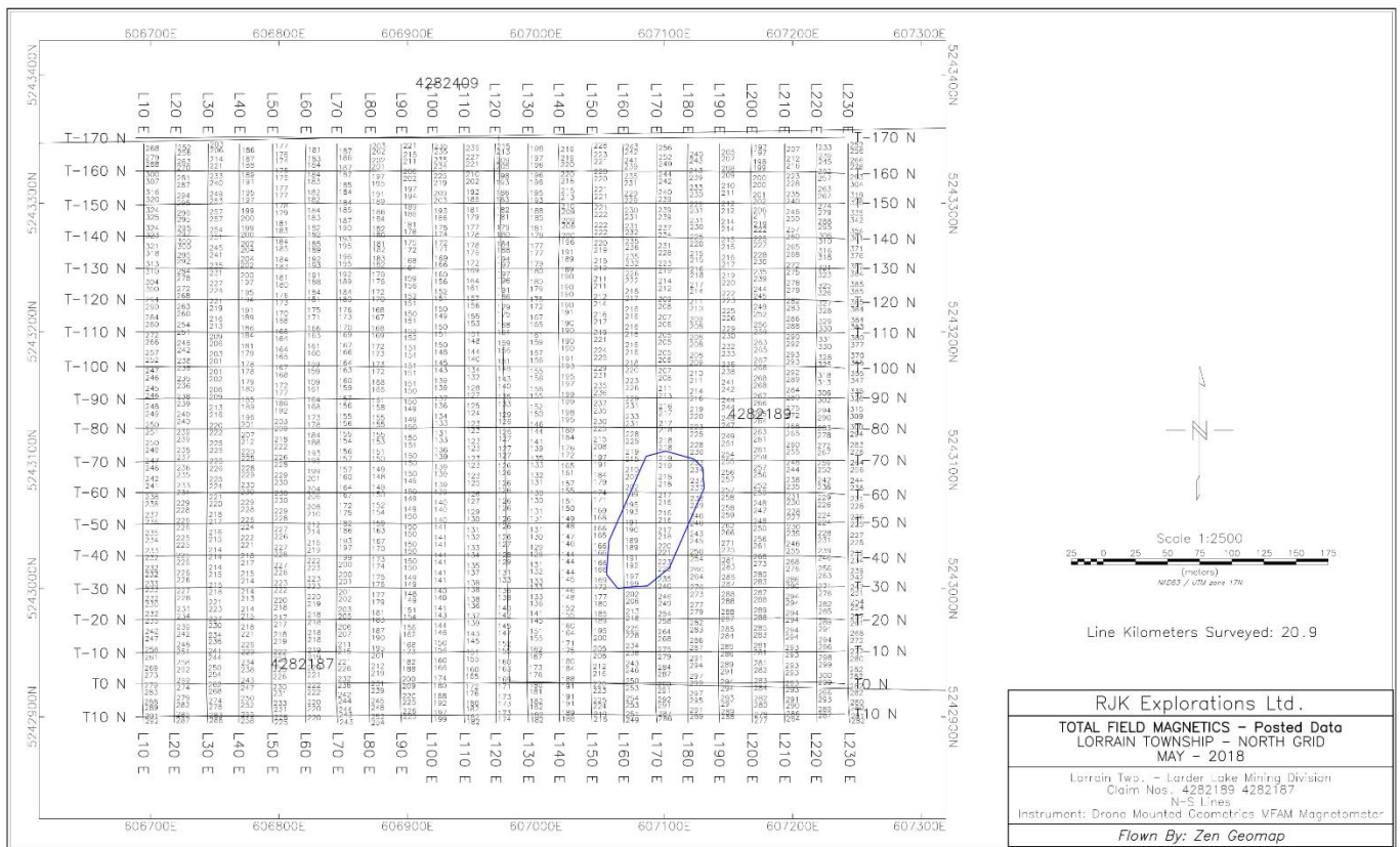
Figure 11: Total Field Magnetics – Posted Data North-South lines, Cedar Pond
