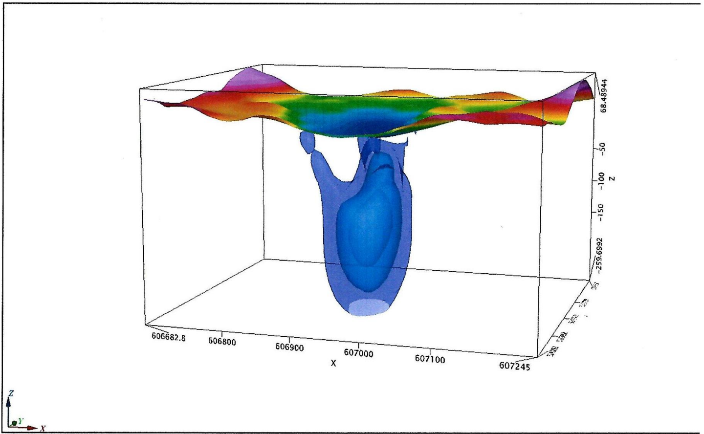
Figure 15: 3D Inversion Model with magnetic overlay looking 343 degrees (NNW) at 10-degree inclination, Cedar Pond
