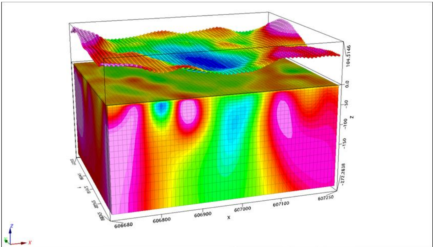
Figure 14: 3D Inversion Voxel with magnetic overlay looking 20 degrees (NNE) at 18-degrees inclination, Cedar Pond
