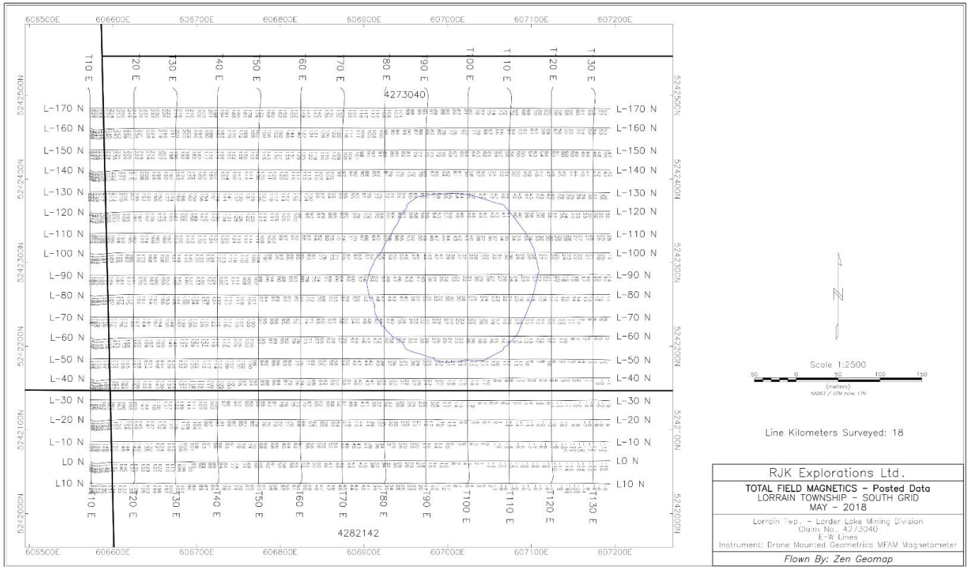
Figure 2: Total Field Magnetics – Posted Data East-West lines, Paradis Pond
