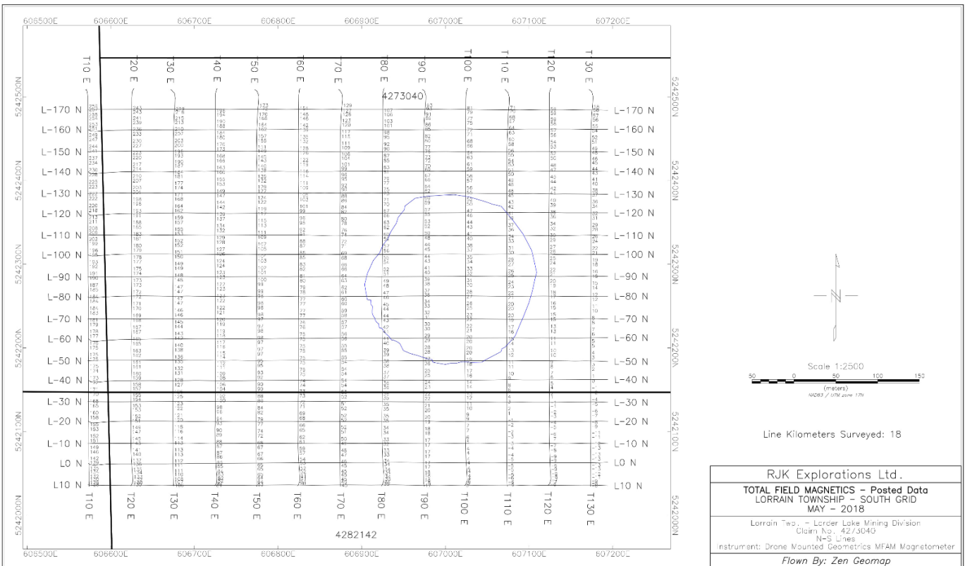
Figure 3: Total Field Magnetics – Posted Data North-South lines, Paradis Pond
