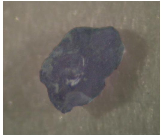
Photos A & B: kimberlitic Cr pyrope photographed under two different LED lights from Trench till sample
