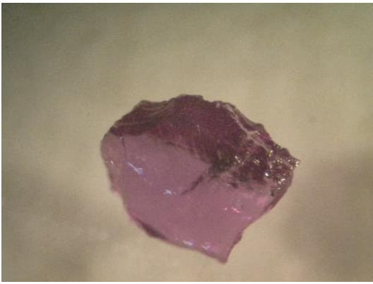
1 - G9 – Cr pyrope – 1.0 x 1.5mm
