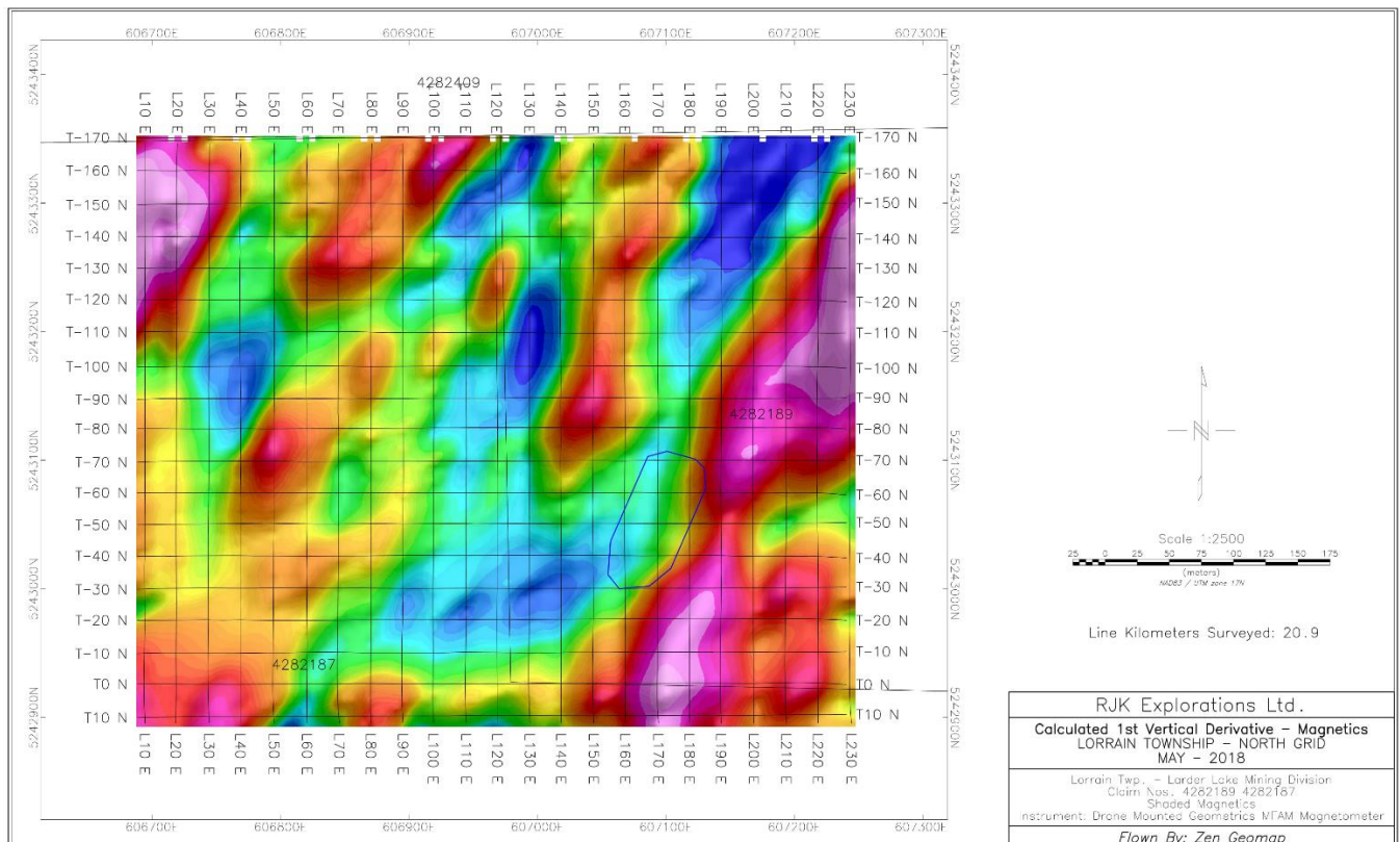
Figure 12: Calculated 1 st Derivative – Magnetics, Cedar Pond
