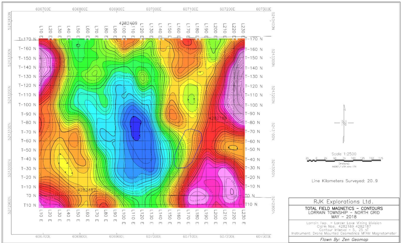
Figure 9: Cedar Pond Total Field Magnetics – contours
