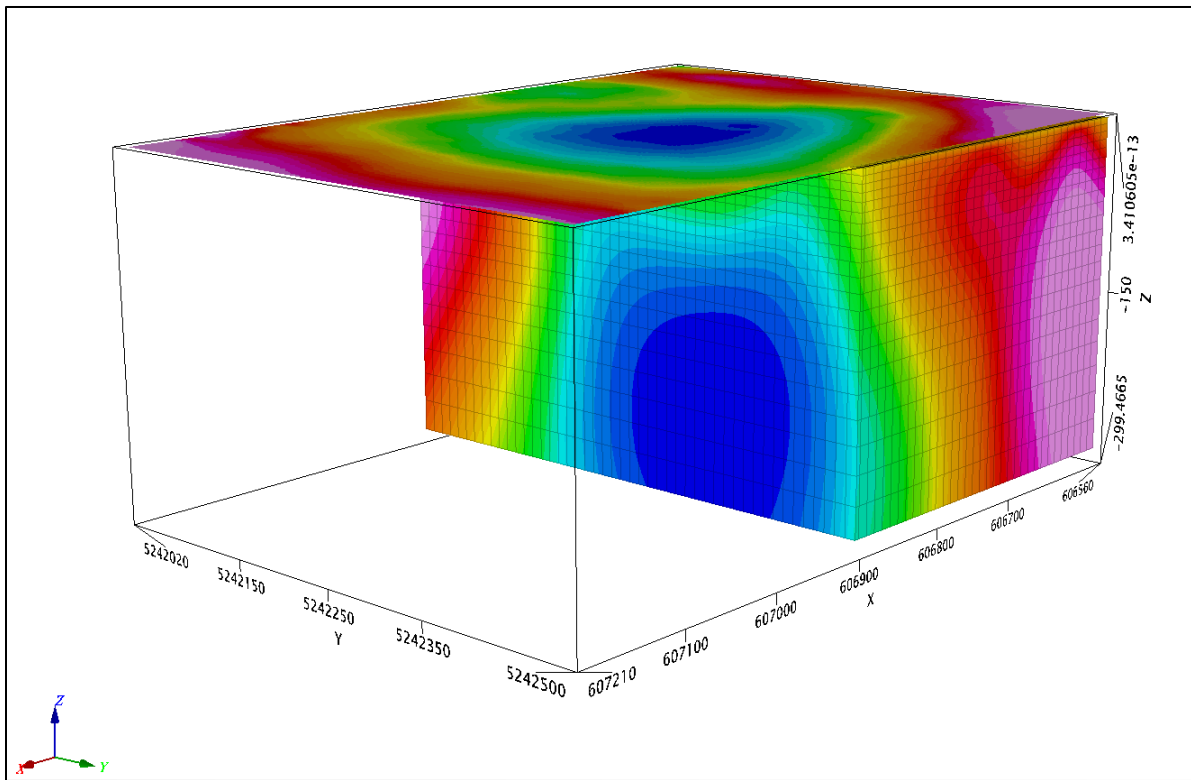
Figure 6: 3D Voxel looking Southwest at inclination 15 degrees (Voxel section cut along 606900E), Paradis Pond
