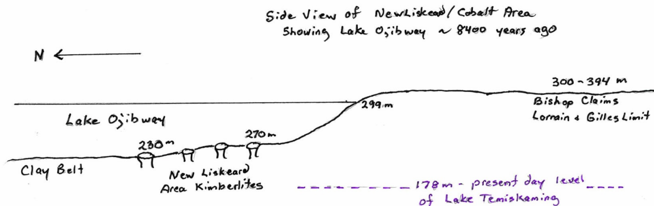
Diagram F – Side view of New Liskeard/Cobalt Area, showing Lake Ojibway ~8400 years ago
