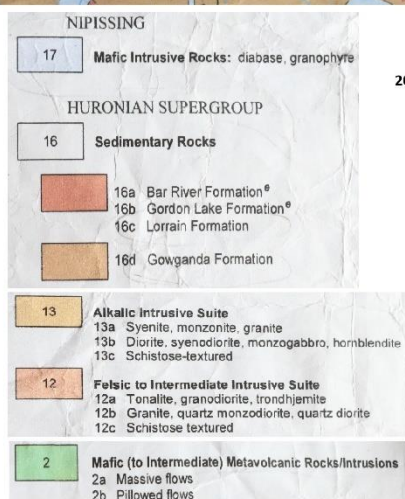
Map 6: Geological Compilation Map (Ayer et al, 2006)
