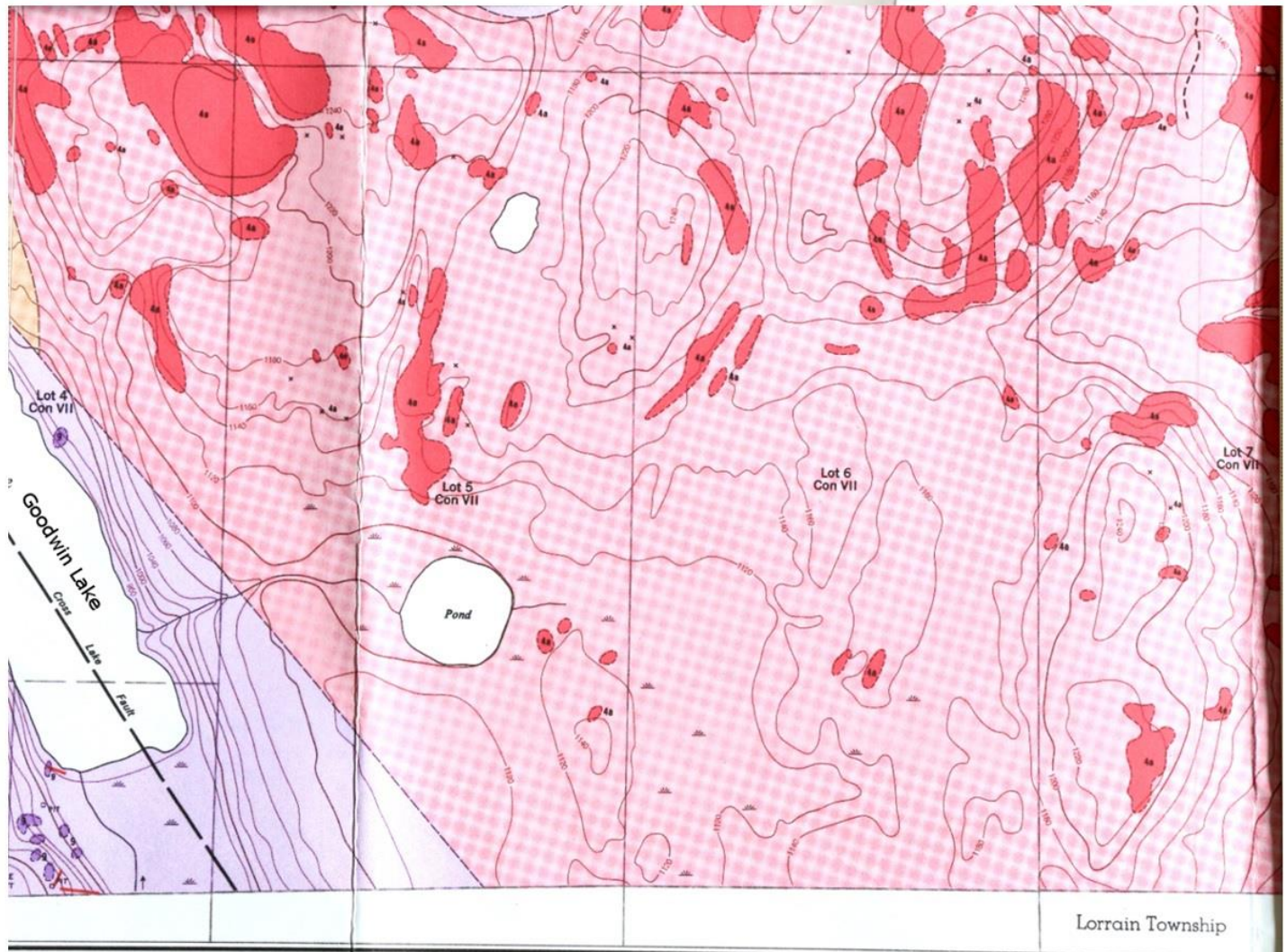
Map 8: Geological Compilation of The Trench area (portion of Ontario Department of Mines Map 2052, 1964)
