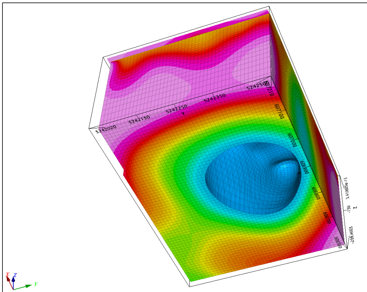
Figure 7: 3D Voxel showing pipe-like structure from below Paradis Pond
