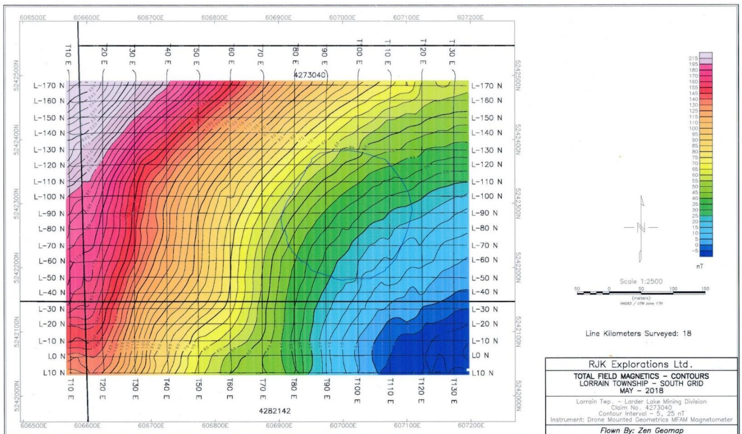
Figure 1: Total Field Magnetics over Paradis Pond
