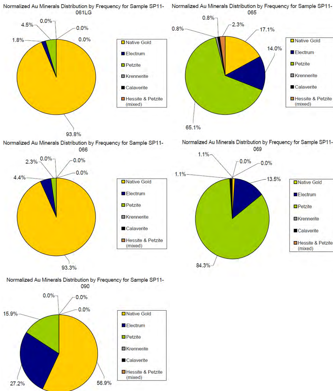
Figure 12.2: Gold Occurrence in Gravity Concentrates
