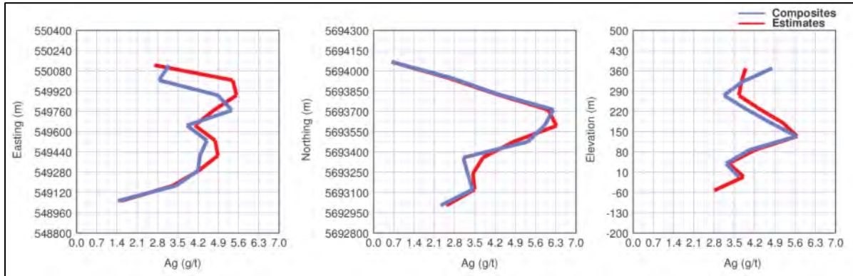
Figure 13.11: Swatch Plot for Silver within the Portage Zone
