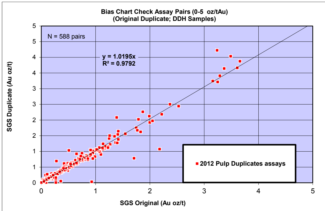
Plots of pulp duplicate samples for 2012 drilling program
