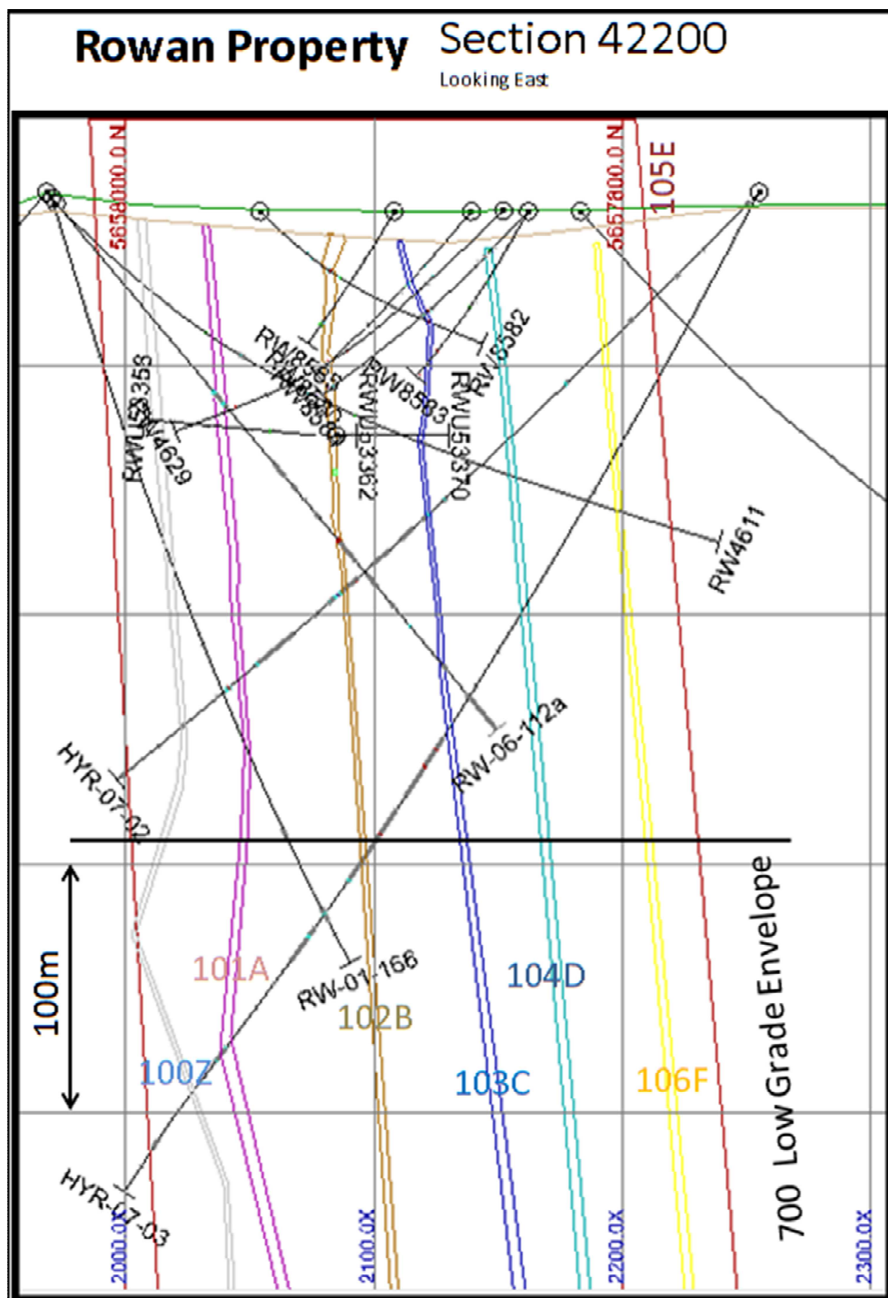
Figure 7 - Section 42200E
